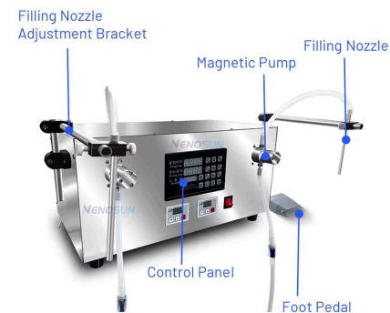
LIQUID FILLING 2 HEAD
